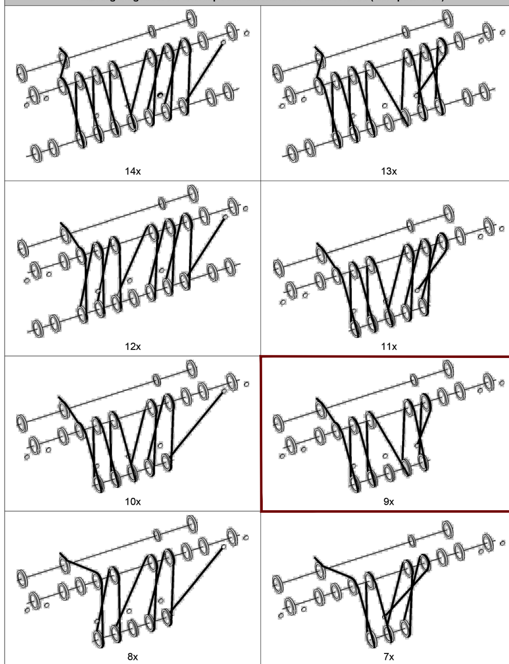
Reeving diagrams for one rope across main boom head 2821 (load position1)
