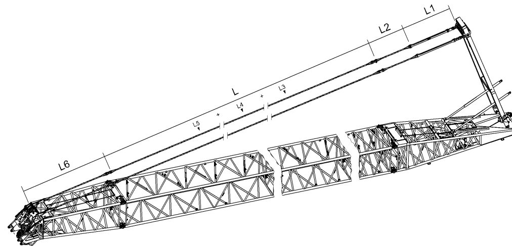
Fig. 2637: Overview of main boom 2821 CF pendant straps
